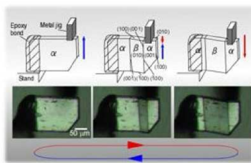
Organosuperelasticity
